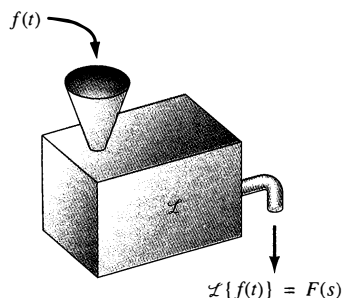
FIGURE 4.1.1. Transformation of a function: \mathcal{L} in analogy with D .
