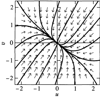
FIGURE 7.4.12. Phase plane portrait for the linear system in Eq. (24) corresponding to the critical point (4, 6).
