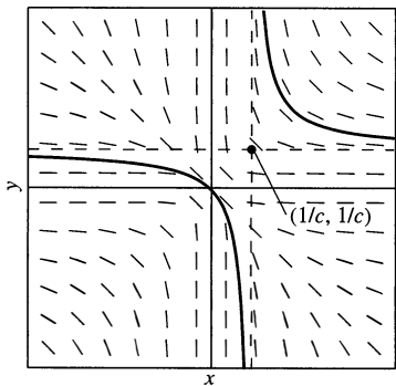
FIGURE 1.3.26. Slope field for x^2y' + y^2 = 0 and graph of a solution y(x) = x/(cx - 1) .
