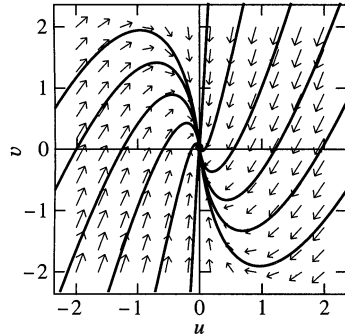
FIGURE 7.4.5. Phase plane portrait for the linear system in Eq. (13) corresponding to the critical point (0, 32) .
